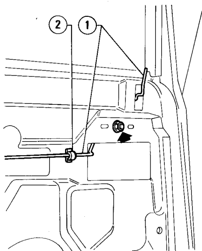
1 Door lock control rod 2 Plastic circlip
