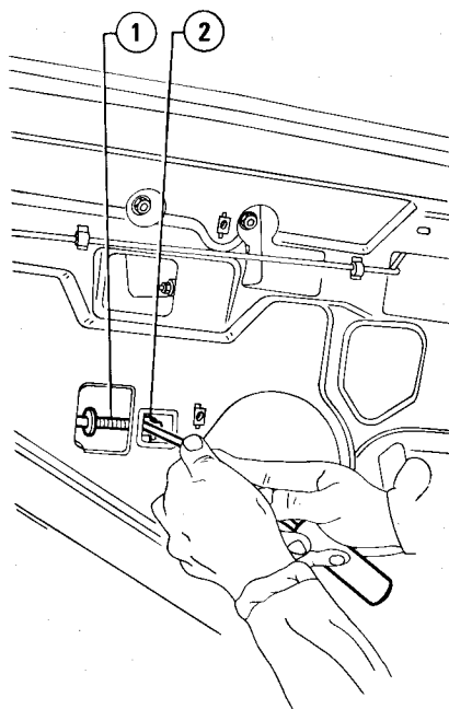
1 Door opening control rod 2 Plastic circlip
